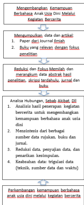
Gambar 1. Alur Penelitian
