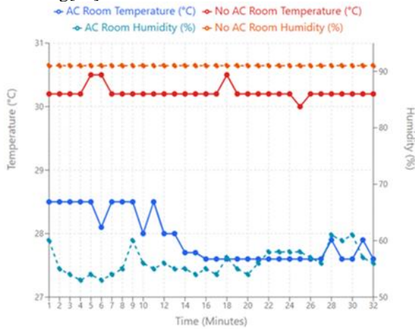
Figure 7. Temperature and humidity consistency test
