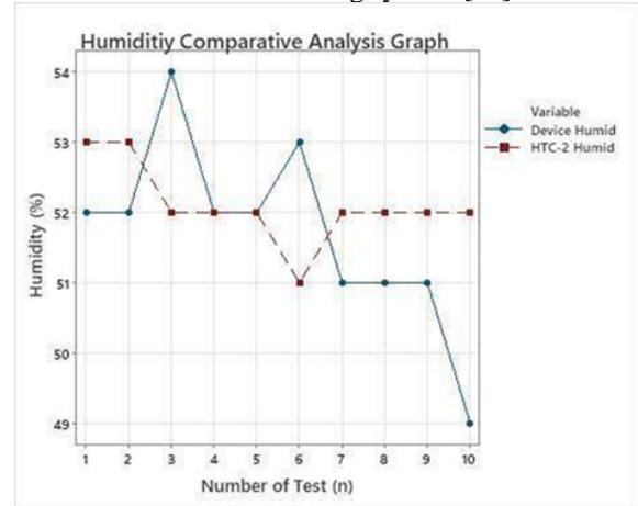
Figure 9. Comparative Humidity Analysis between the DHT11 Sensor Prototype and the HTC-2 Reference Device
