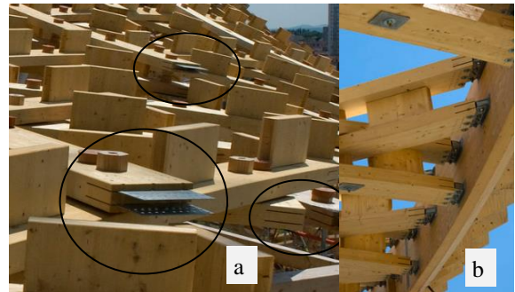
Gambar 15. Penunpu Atap Pompidou Centre Metz Sumber: https://www.centrepompidou-metz.fr
