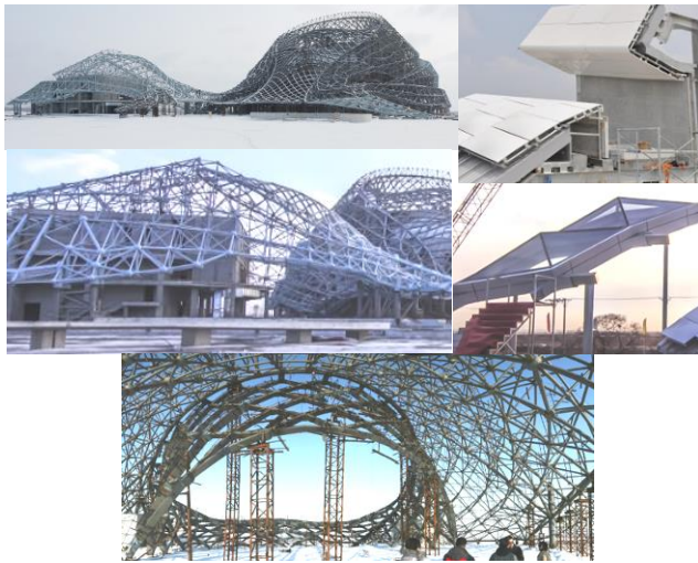
Gambar 22. Konstruksi Atap Harbin Opera House Sumber : https://www.archdaily.com
