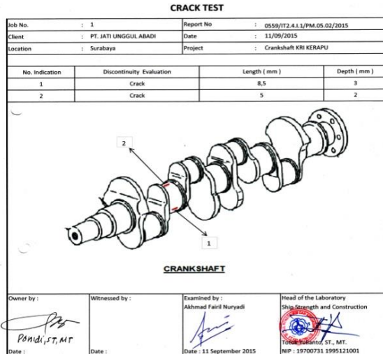
Gambar 2 Hasil Pengukuran Kedalaman keretakan Crankshaft di ITS Surabaya
